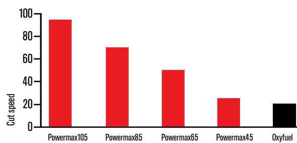
Cut speed comparison on 12 mm mild steel
